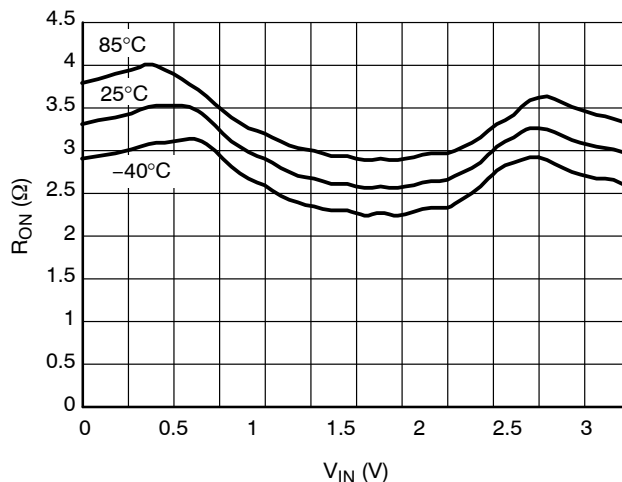
Figure 5. On-Resistance vs. Input Voltage @ V_{CC} = 3.3 V
