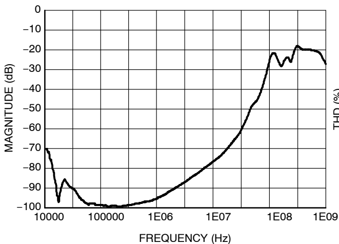
Figure 8. Cross Talk vs. Frequency @ 25^{\circ}C
