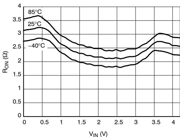
Figure 6. On-Resistance vs. Input Voltage @ V_{CC} = 4.2 V
