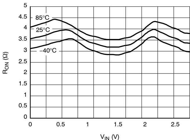
Figure 4. On-Resistance vs. Input Voltage @ V_{CC} = 2.7 V
