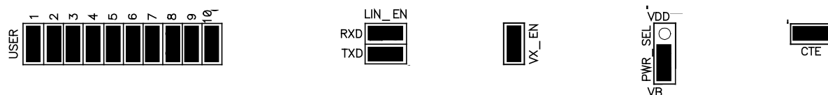
Figure 1: DEMO9S08DZ60 Default Settings
