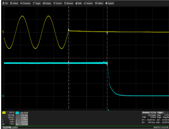
Figure 3: DA45C-J3WUS Hold-up Time (Vo=5V) Vin = 90Vac/63Hz/0° Load: Io = 3A Ch 1: V IN Ch 3: Vo
