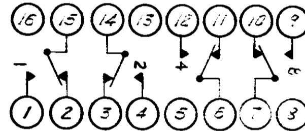
SCHEMATIC (POSITION 0)
