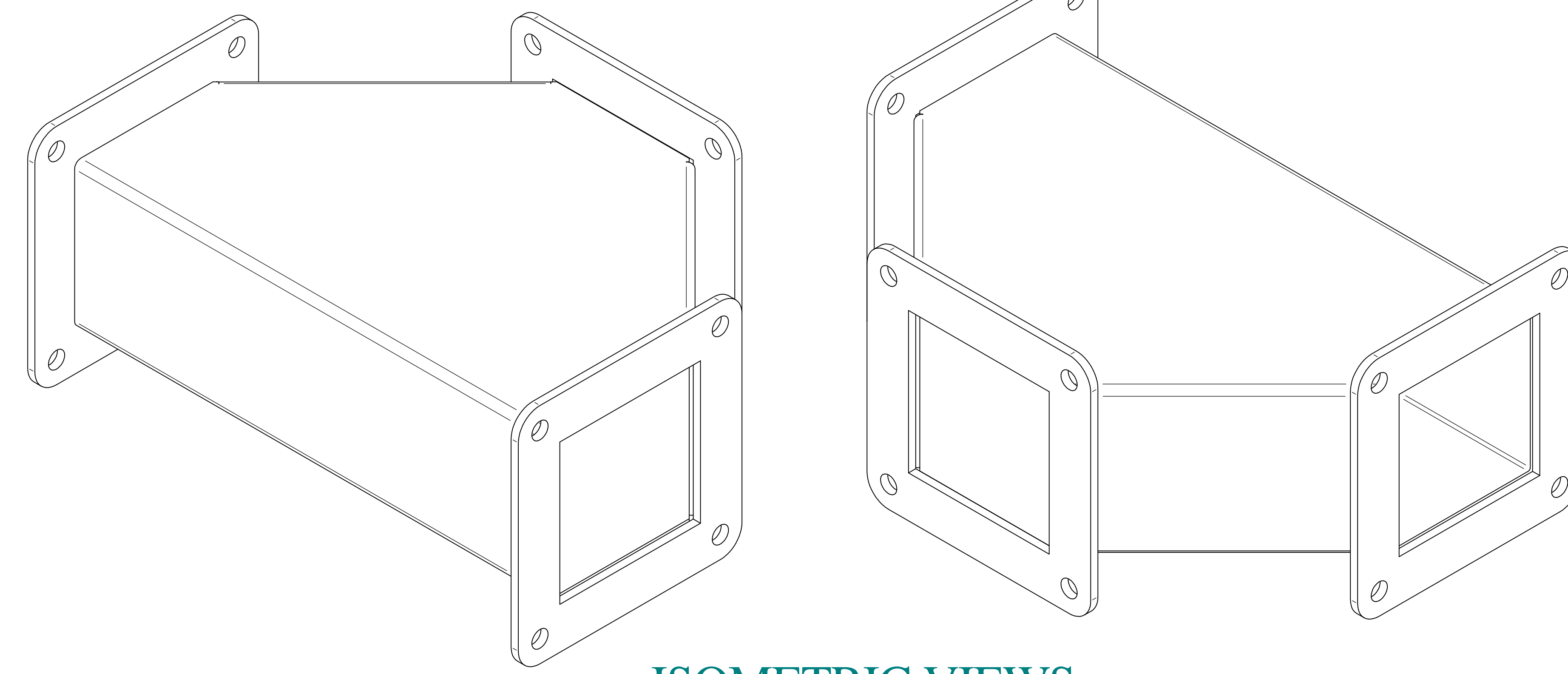
ISOMETRIC VIEWS
