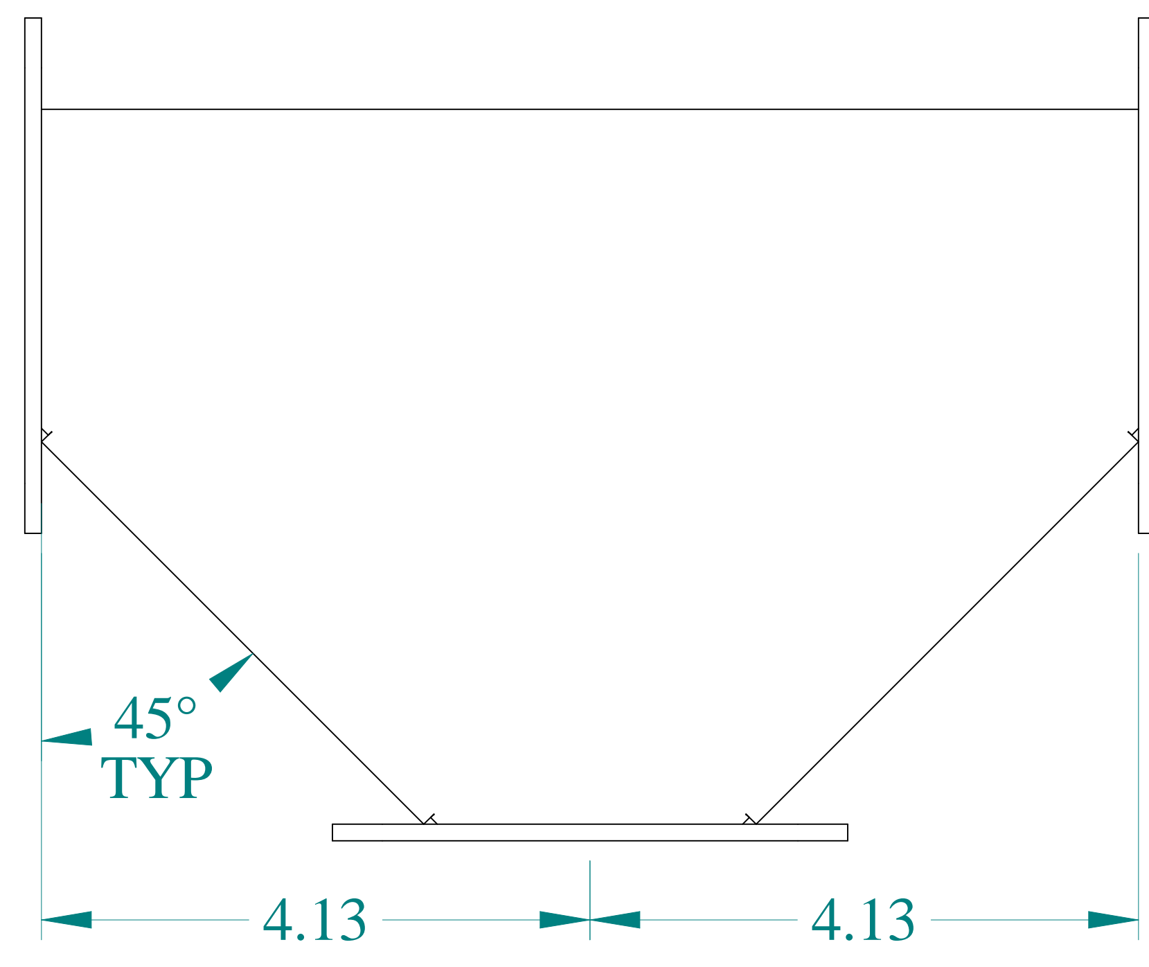
TOP VIEW
