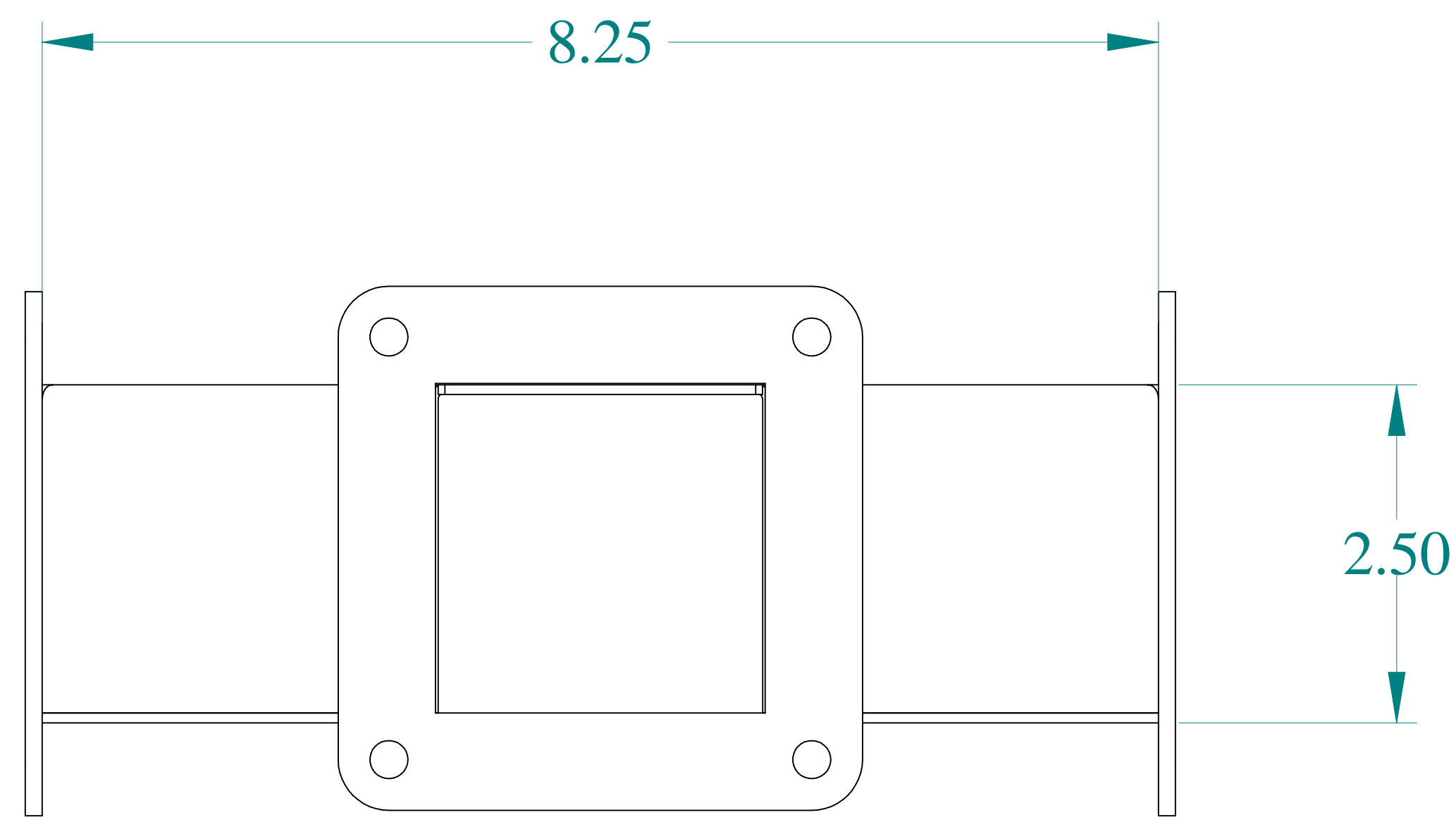
FRONT VIEW
