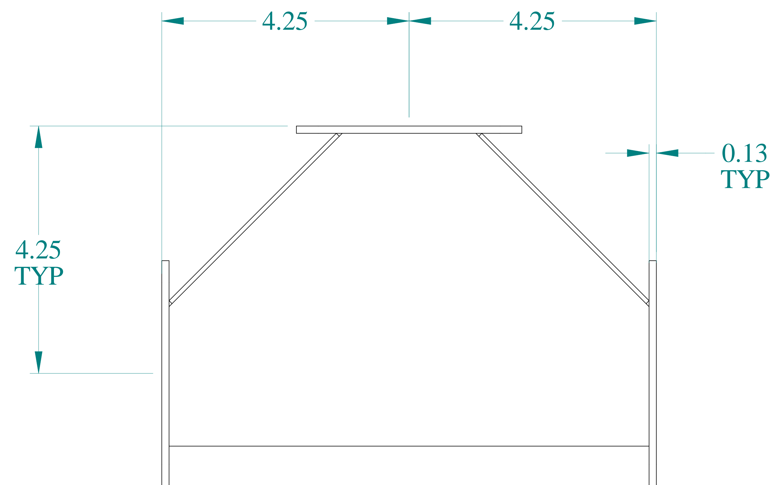
BOTTOM VIEW
