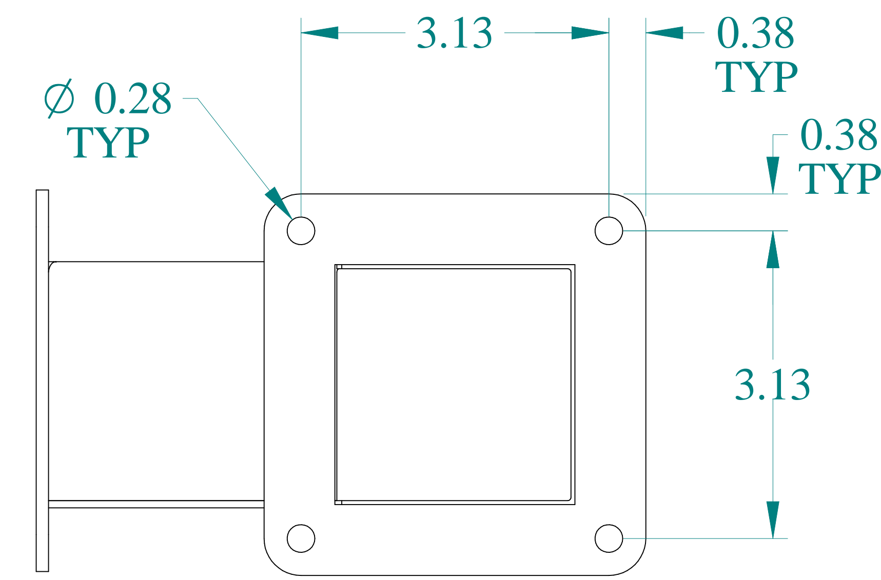
SIDE VIEW
