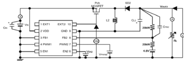
Circuit ⑥
