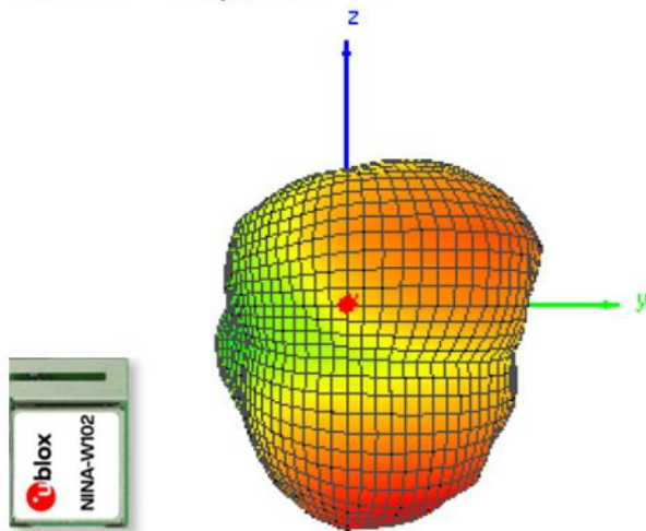
Theta = 90, Phi = 0
