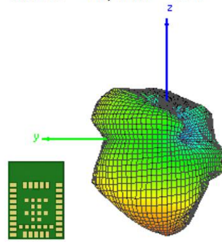
Theta = 90, Phi = 180
