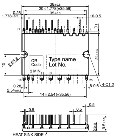
PS2 Super-mini DIIPM™ Ver. 4 PS219**-4C/-CT PS219*3-4CE/-CET
