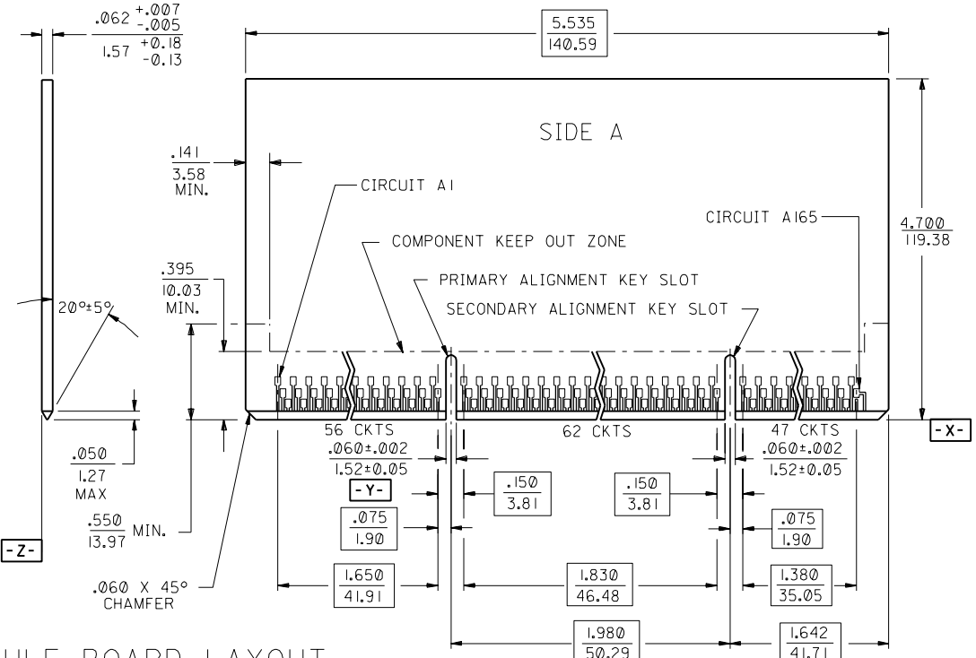
RECOMMENDED MODULE BOARD LAYOUT
