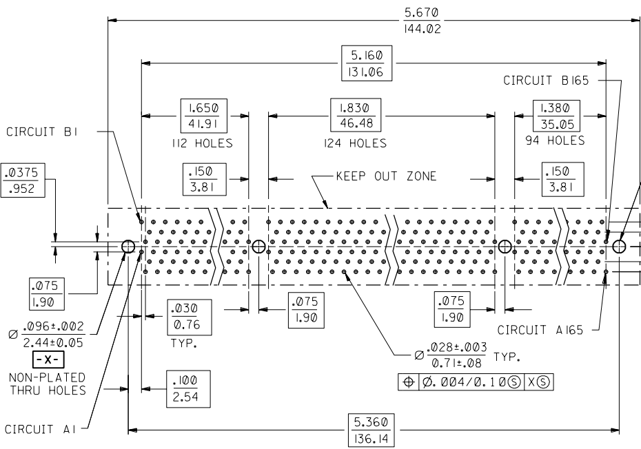
RECOMMENDED PCB HOLE LAYOUT
