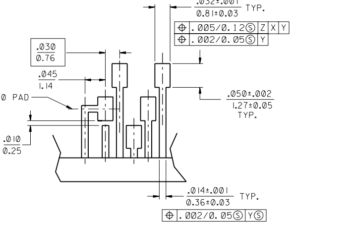
DETAIL Z SCALE 10:1
