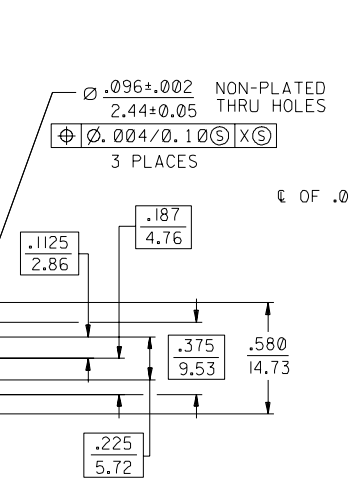
RECOMMENDED MODULE BOARD LAYOUT
