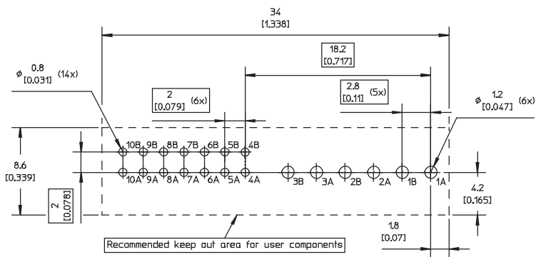
RECOMMENDED FOOTPRINT - TOP VIEW
