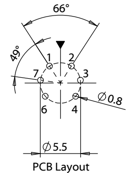
PCB Layout
