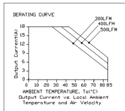
Figure 2. Vin=48 V
