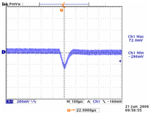
Figure 3. V_{out}=12\text{ V} , 50% to 75% Load Transients at 12 V, T_a = 25^\circ\text{C}
