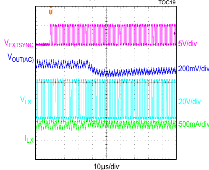
10μs/div CONDITIONS: 62.5Ω LOAD
