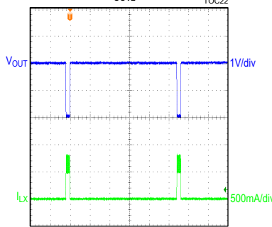
20ms/div CONDITIONS: 5Ω RESISTIVE LOAD
