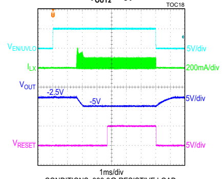
1ms/div CONDITIONS: 333.3Ω RESISTIVE LOAD, RESET IS PULLED UP TO 5V CONNECTED AT VEXT2
