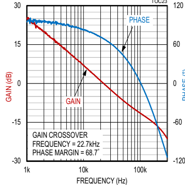
CONDITIONS: 62.5Ω LOAD
