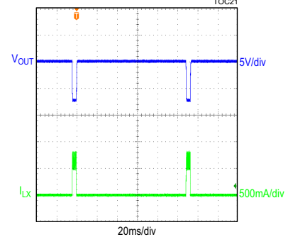
20ms/div CONDITIONS: 20Ω LOAD
