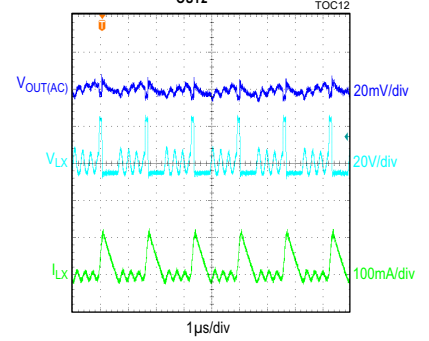
MAX17580 STEADY STATE AT 15mA LOAD VOUT2 = -5V
