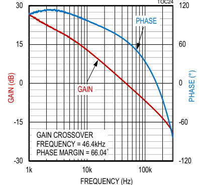
CONDITIONS: 16.67Ω LOAD
