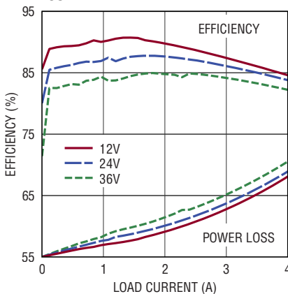
Efficiency and Power Loss V_{OUT} = 1.8\text{V} , BIAS = 5V, Burst Mode
