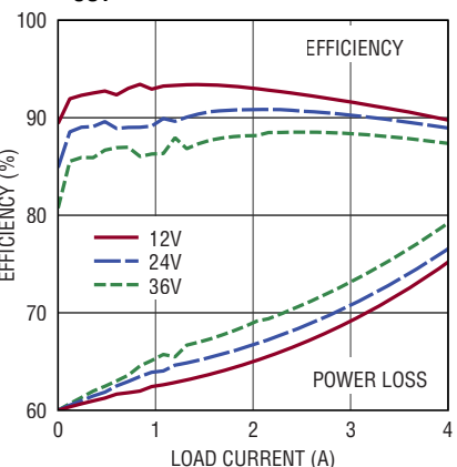
Efficiency and Power Loss V_{OUT} = 3.3\text{V} , BIAS = 5V, Burst Mode
