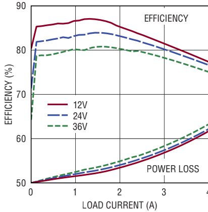
Efficiency and Power Loss V_{OUT} = 1\text{V} , BIAS = 5V, Burst Mode
