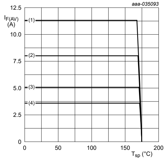
T_j = 175 ^{\circ}C (1) \delta = 1 ; DC (2) \delta = 0.5 ; f = 20 kHz (3) \delta = 0.2 ; f = 20 kHz (4) \delta = 0.1 ; f = 20 kHz
