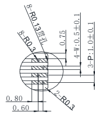
Detail A SCALE 3:1
