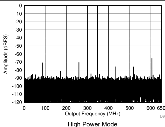
Figure 7-4. Single Tone FFT at 347 MHz and -1 dBFS
