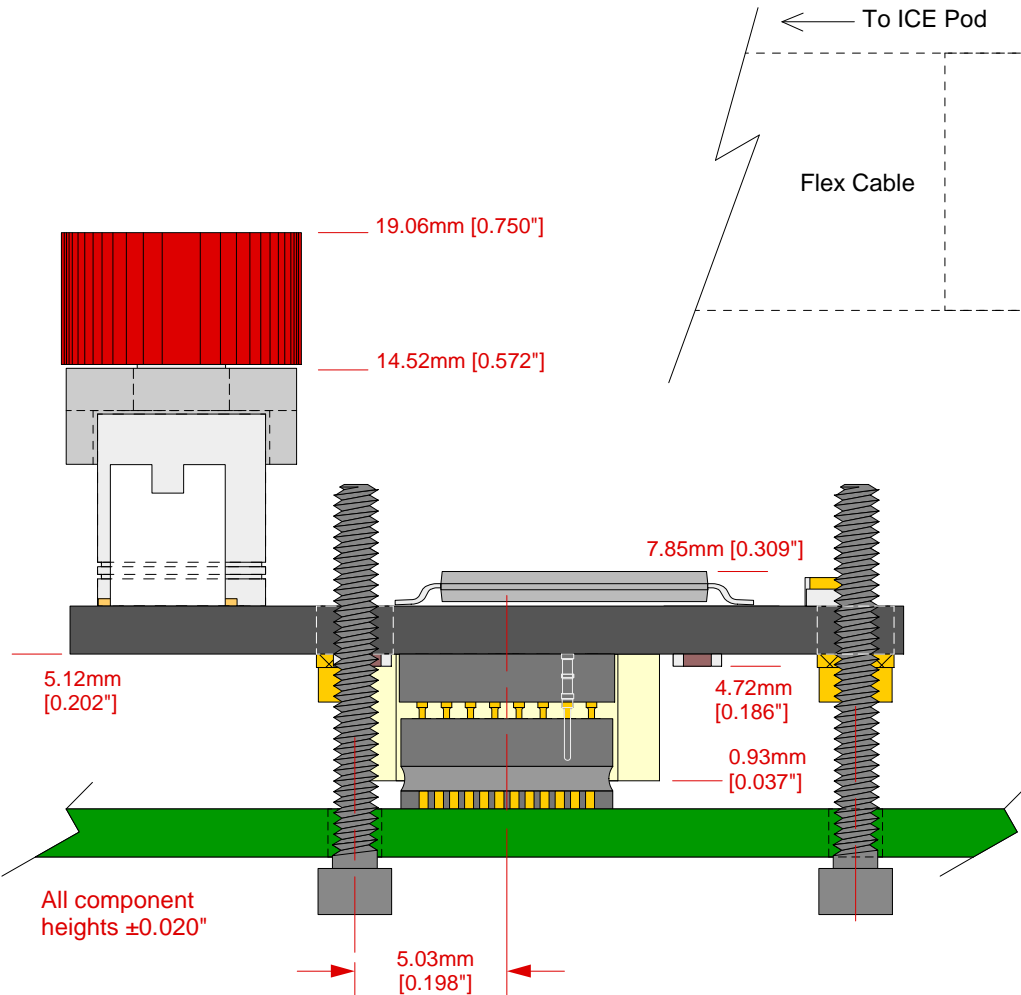
Side view: CY3250-286XXQFN Pod on QFN48 foot
