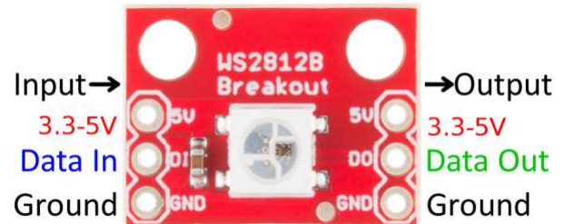
WS2812B breakout board's pinout.
