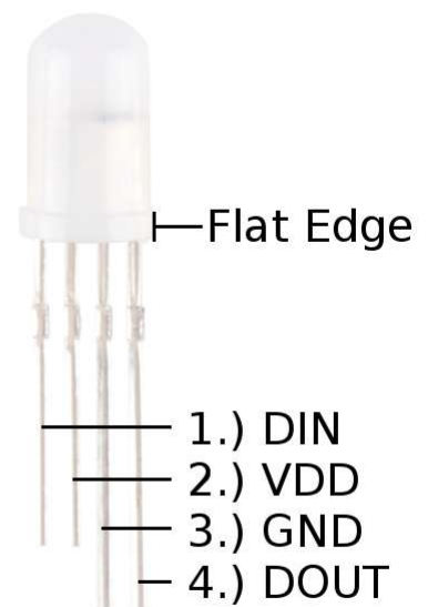
Diffused Addressable 5mm LED
