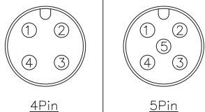
Pin Assignments Front View
