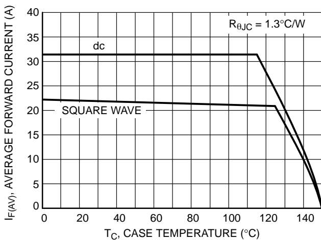
Figure 5. Current Derating
