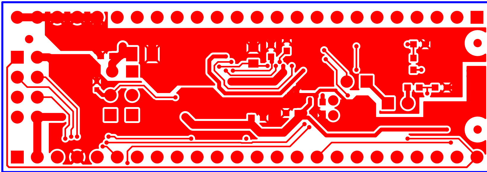
EVAL-ADuCM362/363QSPZ (Rev. A) - 08_042342a - Top Side View. Bottom Side - Layer 2
