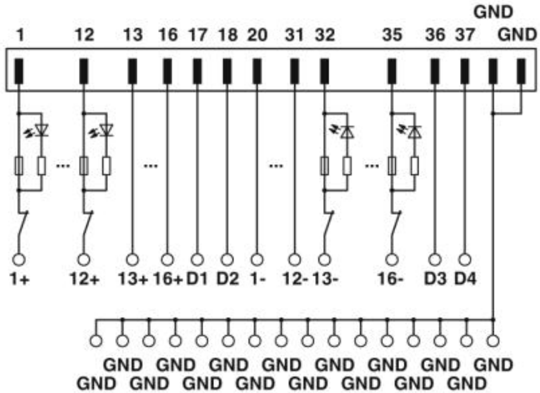
Circuit diagram
