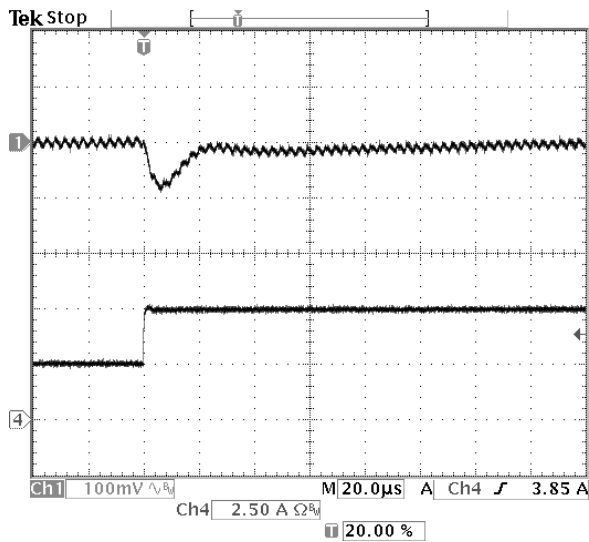
Fig-3.3V-6: Output voltage response for V_{out}=3.3V to positive load current step-change from 2.5A to 5A with slew rate of 5A/\mu s at V_{in}=5.0V . C_o=47\mu F \times 2 ceramic. Top trace: output voltage (100mV/div.) Bottom trace: load current (2.5A/div.) Time scale: 20μs/div.
