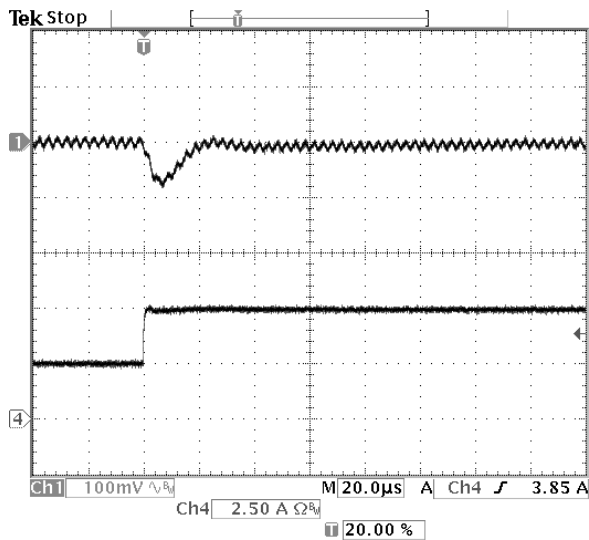
Fig-2.0V-6: Output voltage response for V_{out}=2.0V to positive load current step-change from 2.5A to 5A with slew rate of 5A/\mu s at V_{in}=5.0V . C_o=47\mu F \times 2 ceramic. Top trace: output voltage (100mV/div.) Bottom trace: load current (2.5A/div.) Time scale: 20μs/div.
