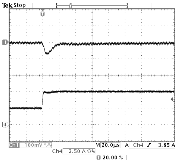
Fig-0.7525V-6: Output voltage response for V_{out}=0.7525V to positive load current step-change from 2.5A to 5A with slew rate of 5A/\mu s at V_{in}=5.0V . C_o=47\mu F \times 2 ceramic. Top trace: output voltage (100mV/div.) Bottom trace: load current (2.5A/div.) Time scale: 20μs/div.
