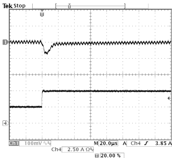
Fig-2.5V-6: Output voltage response for V_{out}=2.5V to positive load current step-change from 2.5A to 5A with slew rate of 5A/\mu s at V_{in}=5.0V . C_o=47\mu F \times 2 ceramic.
