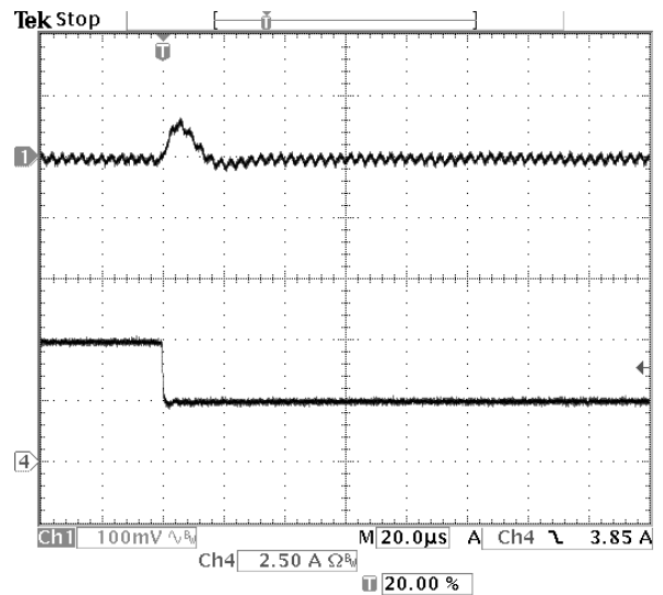
Fig-1.5V-7: Output voltage response for V_{out}=1.5V to positive load current step-change from 5A to 2.5A with slew rate of -5A/\mu s at V_{in}=5.0V . C_o=47\mu F \times 2 ceramic.
