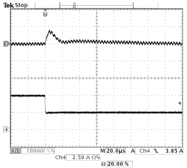
Fig-3.3V-7: Output voltage response for V_{out}=3.3V to negative load current step-change from 5A to 2.5A with slew rate of -5A/\mu s at V_{in}=5.0V . C_o=47\mu F \times 2 ceramic. Top trace: output voltage (100mV/div.) Bottom trace: load current (2.5A/div.) Time scale: 20μs/div.
