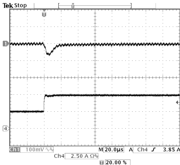
Fig-1.0V-6: Output voltage response for V_{out}=1.0V to positive load current step-change from 2.5A to 5A with slew rate of 5A/\mu s at V_{in}=5.0V . C_o=47\mu F \times 2 ceramic.
