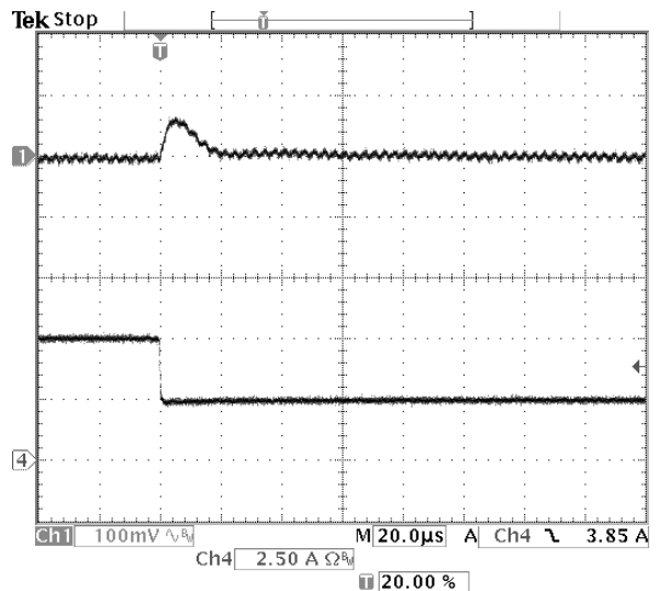
Fig-0.7525V-7: Output voltage response for V_{out}=0.7525V to positive load current step-change from 5A to 2.5A with slew rate of -5A/\mu s at V_{in}=5.0V . C_o=47\mu F \times 2 ceramic. Top trace: output voltage (100mV/div.) Bottom trace: load current (2.5A/div.) Time scale: 20μs/div.
