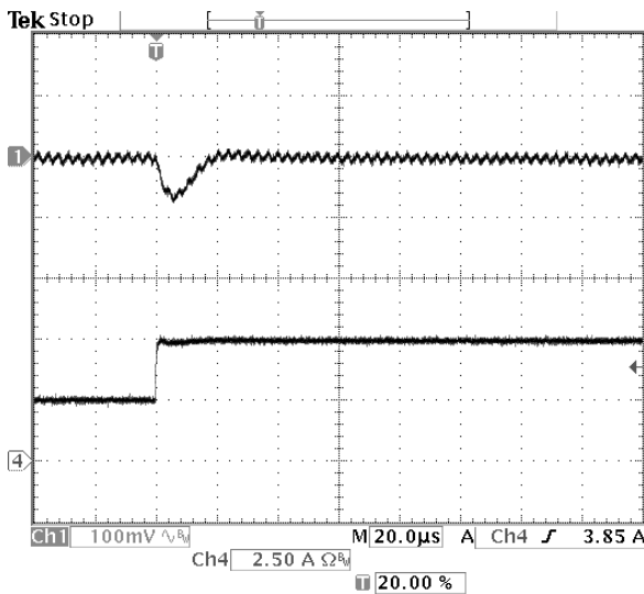
Fig-1.5V-6: Output voltage response for V_{out}=1.5V to positive load current step-change from 2.5A to 5A with slew rate of 5A/\mu s at V_{in}=5.0V . C_o=47\mu F \times 2 ceramic.
