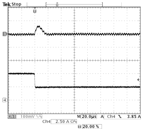
Fig-1.2V-7: Output voltage response for V_{out}=1.2V to positive load current step-change from 5A to 2.5A with slew rate of -5A/\mu s at V_{in}=5.0V . C_o=47\mu F \times 2 ceramic.
