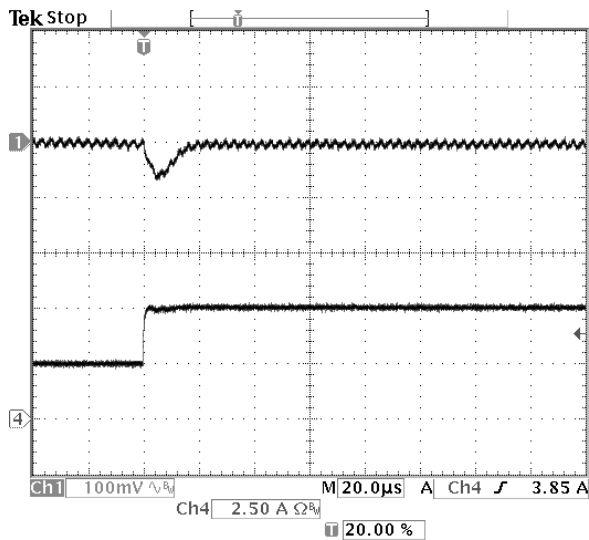
Fig-1.2V-6: Output voltage response for V_{out}=1.2V to positive load current step-change from 2.5A to 5A with slew rate of 5A/\mu s at V_{in}=5.0V . C_o=47\mu F \times 2 ceramic.
