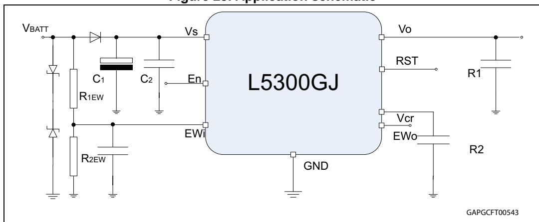
Figure 23. Application schematic
