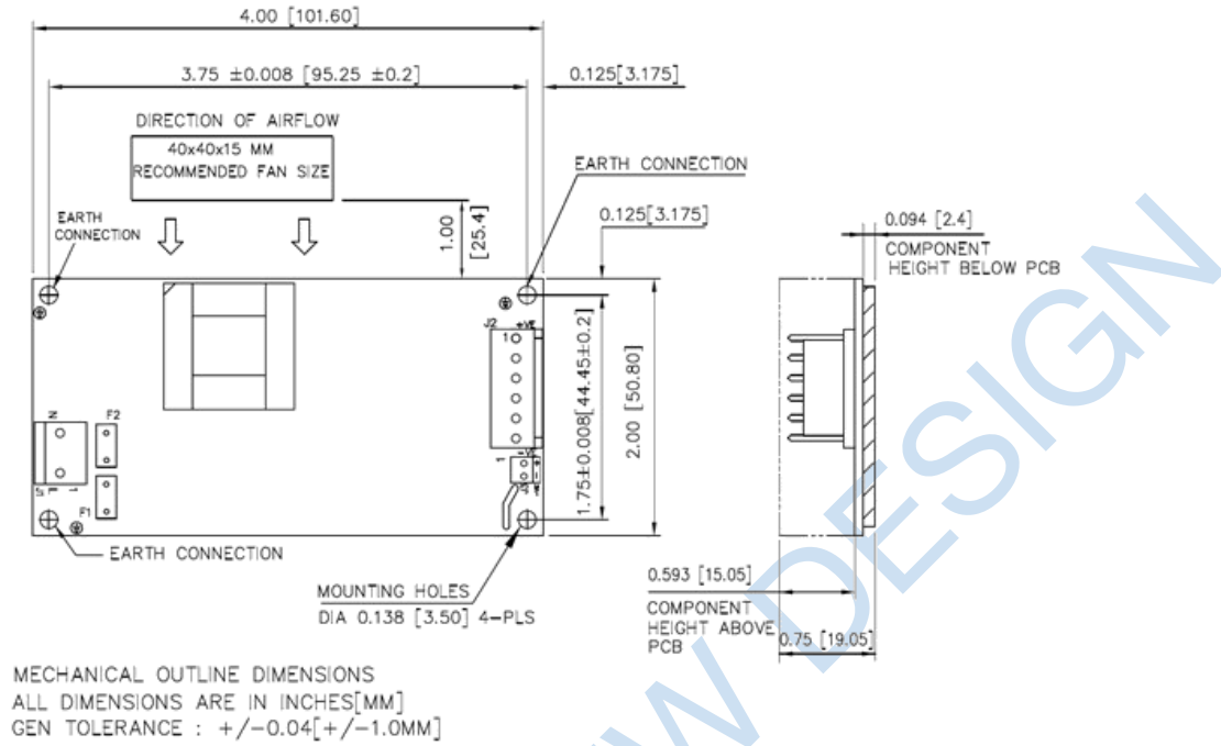
Figure 3. Mechanical Drawing – Option 2 (Output Connector – Header Molex)
