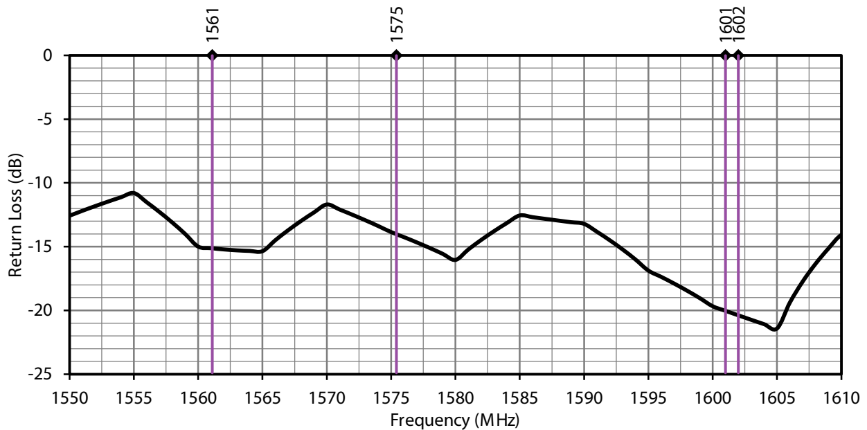
Figure 3. ANT-GNCP-C357L160 Return Loss
