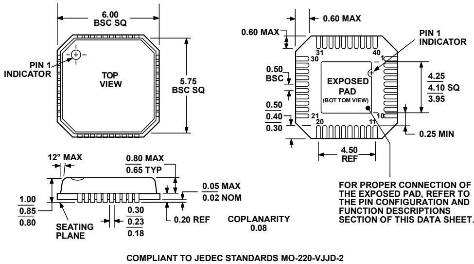
Figure 113. 40-Lead Lead Frame Chip Scale Package [LFCSP] 6 mm x 6 mm and 0.85 mm Package Height (CP-40-1) Dimensions shown in millimeters
