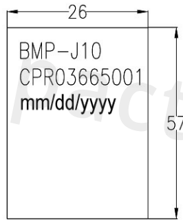
LABEL DETAIL
