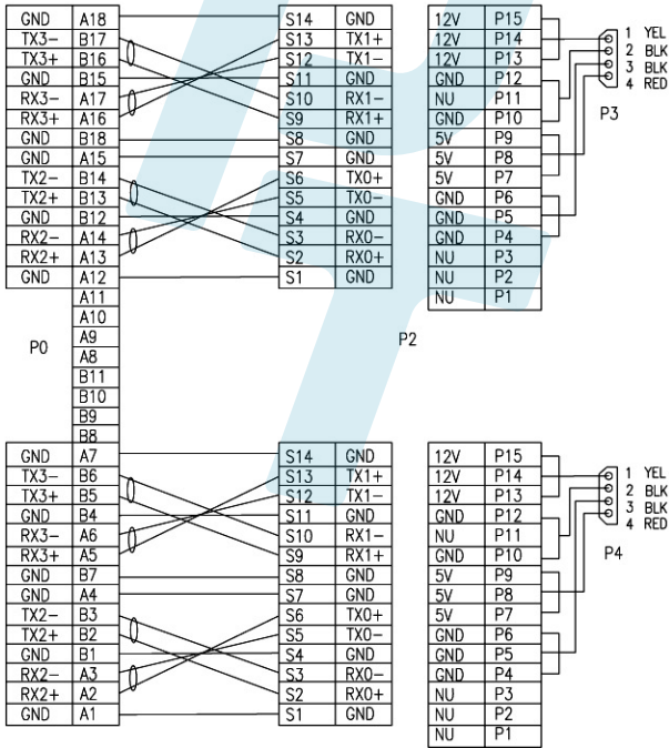
WIRING DIAGRAM
