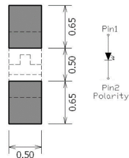
Figure 1. IN-S42CTQHIR Solder Pattern
