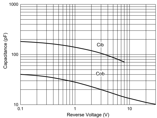
Fig. 6 - C_{ob}/C_{ib} - V_{CB}/V_{EB}
