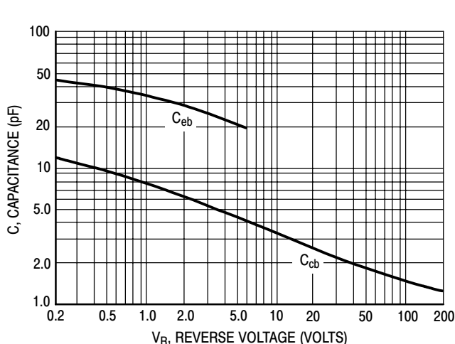
Figure 2. Capacitances
