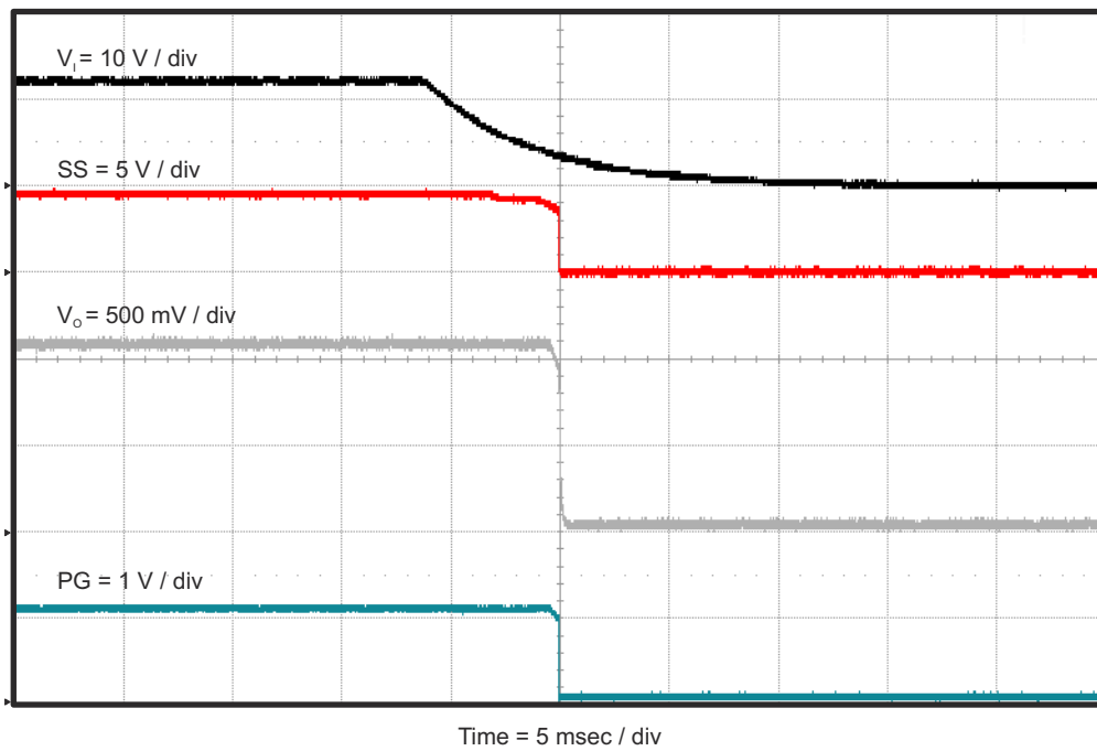
Figure 4-13. TPS562210EVM-663 Shut-Down Relative to V_{IN}
