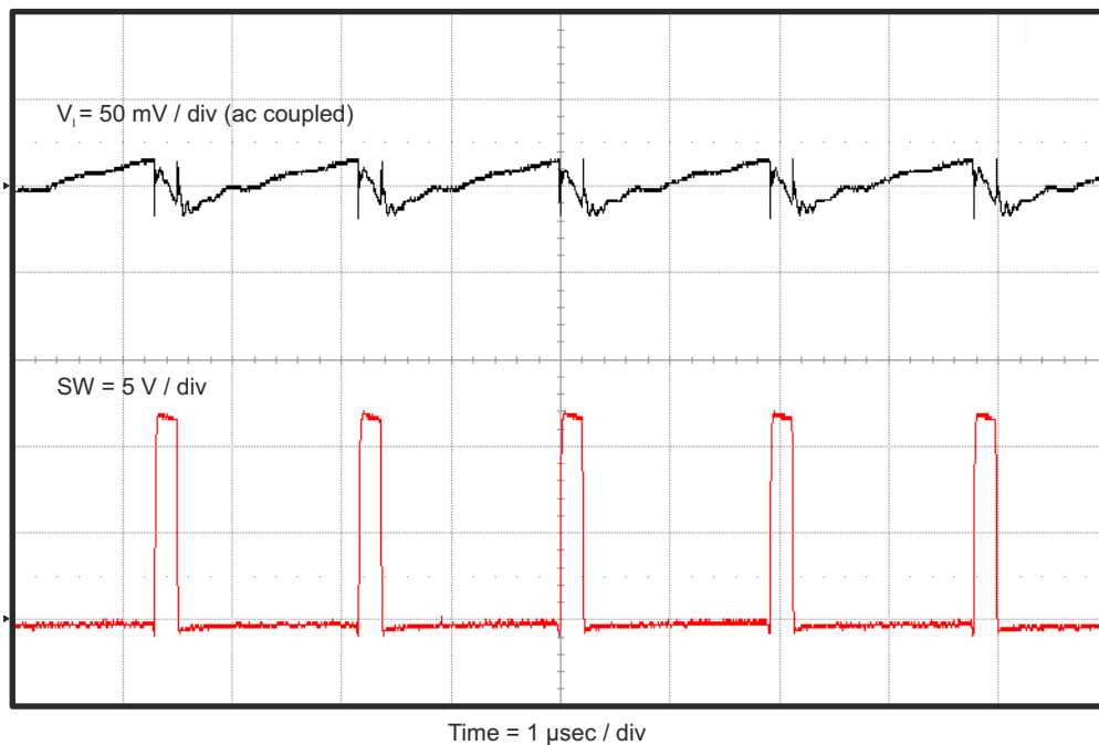
Figure 4-10. TPS562210EVM-663 Input Voltage Ripple, I_{OUT} = 2 A
