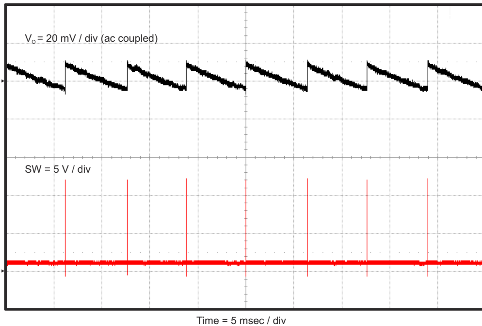
Figure 4-9. TPS562210EVM-663 Output Voltage Ripple, I_{OUT} = 0 mA
