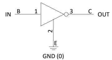
Equivalent Inverter Circuit
