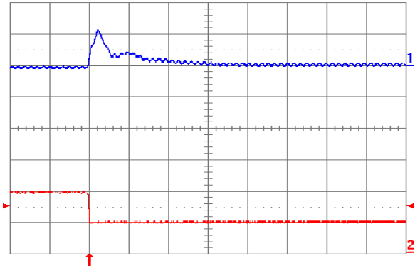
Fig. 1.0V.8: Output voltage response (YNV05T10010) to negative load current step change from 5A to 2.5A with slew rate of -5A/\mu s at V_{in} = 5V . Top trace: output voltage (100mV/div.); Bottom trace: load current (5A/div.). C_o = 100\mu F ceramic + 1\mu F ceramic. Time scale: 20\mu s /div.
