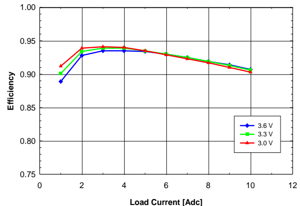
Fig. 1.5V.4: Efficiency vs. load current and input voltage for YNV05T10015 converter mounted vertically with air flowing from pin 10 to pin 1 at a rate of 200 LFM (1m/s) and T_a = 25^\circ C .
