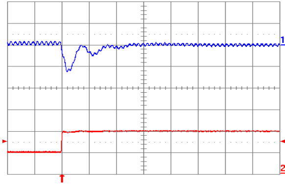
Fig. 1.8V.7: Output voltage response (YNV05T10018) to positive load current step change from 2.5A to 5A with slew rate of 5A/\mu s at V_{in} = 5V . Top trace: output voltage (100mV/div.); Bottom trace: load current (5A/div.). C_o = 100\mu F ceramic + 1\mu F ceramic. Time scale: 20\mu s/div.
