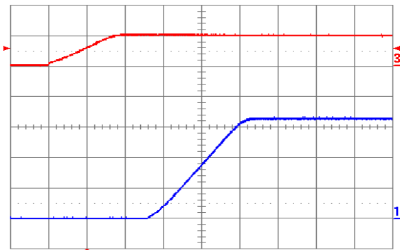
Fig. 3.3V.5: Turn-on transient (YNV05T10033) with application of V_{in} at full rated load current (resistive) and 47\mu F external capacitance at V_{in} = 5V . Top trace: V_{in} (5V/div.); Bottom trace: output voltage (1V/div.); Time scale: 2ms/div.
