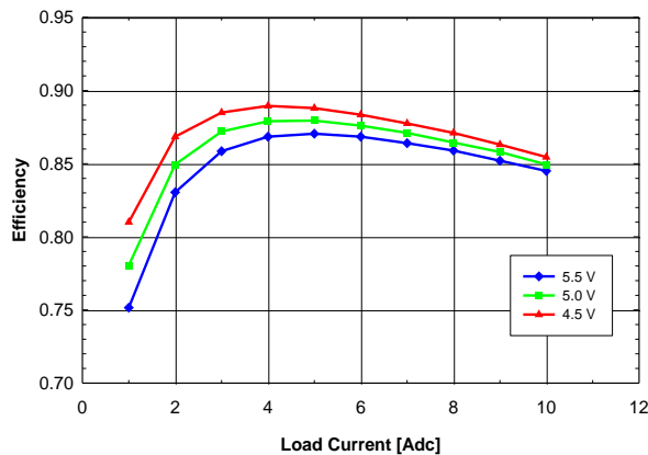
Fig. 0.9V.3: Efficiency vs. load current and input voltage for YNV05T10009 converter mounted vertically with air flowing from pin 10 to pin 1 at a rate of 200 LFM (1m/s) and T_a = 25^\circ C .
