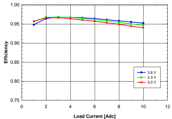
Fig. 2.5V.4: Efficiency vs. load current and input voltage for YNV05T10025 converter mounted vertically with air flowing from pin 10 to pin 1 at a rate of 200 LFM (1m/s) and T_a = 25^\circ C .
