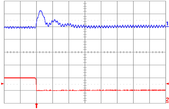
Fig. 1.8V.8: Output voltage response (YNV05T10018) to negative load current step change from 5A to 2.5A with slew rate of -5A/\mu s at V_{in} = 5V . Top trace: output voltage (100mV/div.); Bottom trace: load current (5A/div.). C_o = 100\mu F ceramic + 1\mu F ceramic. Time scale: 20\mu s/div.
