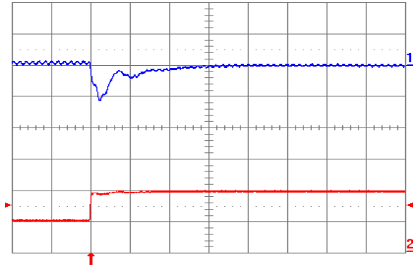
Fig. 1.0V.7: Output voltage response (YNV05T10010) to positive load current step change from 2.5A to 5A with slew rate of 5A/\mu s at V_{in} = 5V . Top trace: output voltage (100mV/div.); Bottom trace: load current (5A/div.). C_o = 100\mu F ceramic + 1\mu F ceramic. Time scale: 20\mu s /div.
