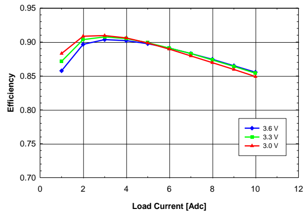
Fig. 0.9V.4: Efficiency vs. load current and input voltage for YNV05T10009 converter mounted vertically with air flowing from pin 10 to pin 1 at a rate of 200 LFM (1m/s) and T_a = 25^\circ C .
