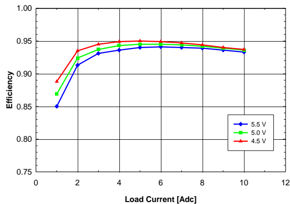
Fig. 2.5V.3: Efficiency vs. load current and input voltage for YNV05T10025 converter mounted vertically with air flowing from pin 10 to pin 1 at a rate of 200 LFM (1m/s) and T_a = 25^\circ C .
