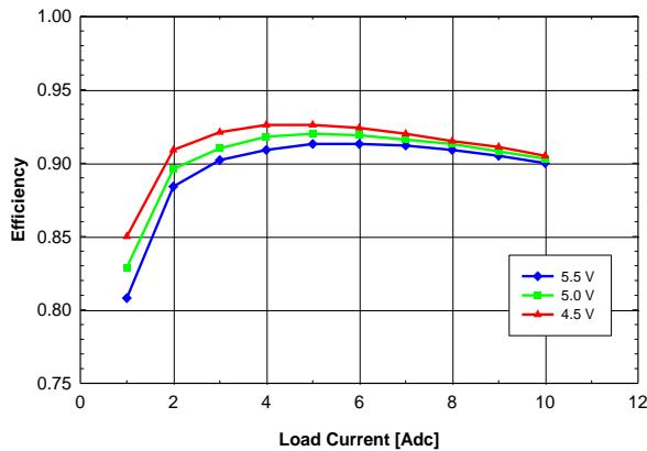
Fig. 1.5V.3: Efficiency vs. load current and input voltage for YNV05T10015 converter mounted vertically with air flowing from pin 10 to pin 1 at a rate of 200 LFM (1m/s) and T_a = 25^\circ C .
