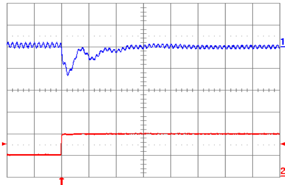
Fig. 2.5V.7: Output voltage response (YNV05T10025) to positive load current step change from 2.5A to 5A with slew rate of 5\text{A}/\mu\text{s} at V_{in} = 5\text{V} . Top trace: output voltage (100mV/div.); Bottom trace: load current (5A/div.). C_o = 100\mu\text{F} ceramic + 1\mu\text{F} ceramic. Time scale: 20μs/div.
