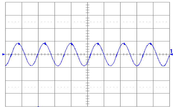
Fig. 3.3V.6: Output voltage ripple (20mV/div.) at full rated load current into a resistive load with external capacitance 47\mu F ceramic + 1\mu F ceramic and V_{in} = 5V (YNV05T10033). Time scale: 2μs/div.
