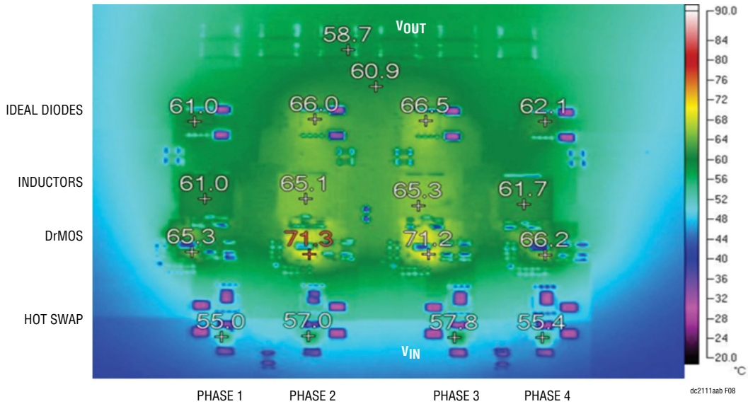
Figure 8. Thermal Image of the 1.2V/90A Converter with N+1 MOSFET Failure Protection. Measured with Full Load and an Input Voltage of 12V. T_{AMB} = 21^{\circ}C . Hot Spot is the DrMOS of Phases 2 with a Rise Over Ambient of 50^{\circ}C .
