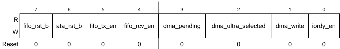
Figure 23-39. ATA_Control Register
