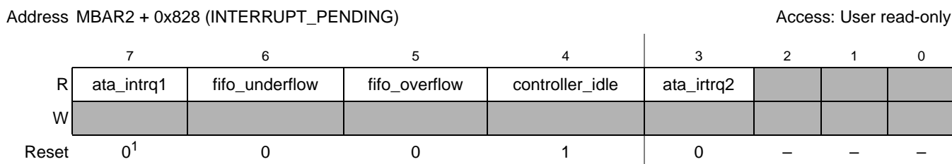
Figure 23-40. Interrupt_Pending Register
