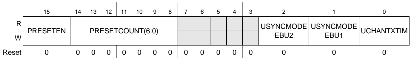
Figure 17-11. CDTEXTCONTROL Register
