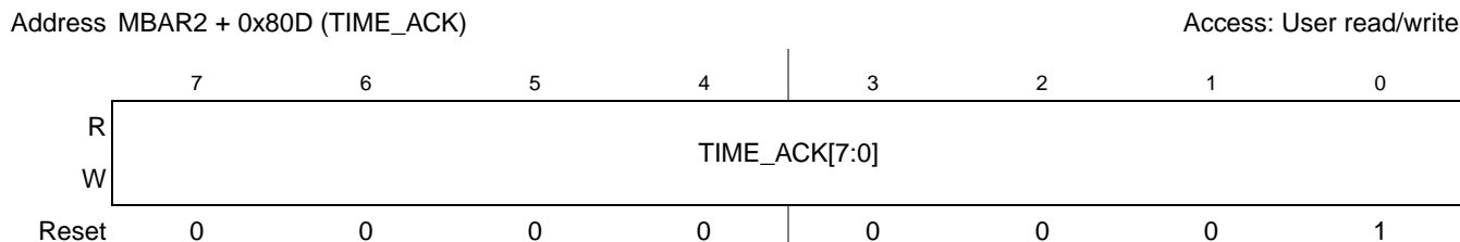
Figure 23-25. TIME_ACK Register
