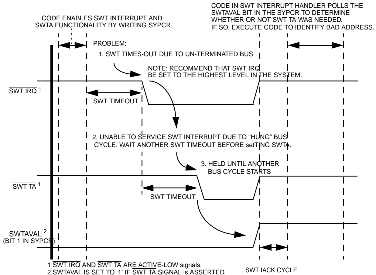
Figure 9-10. MCF5253 Underminated Access Recovery
