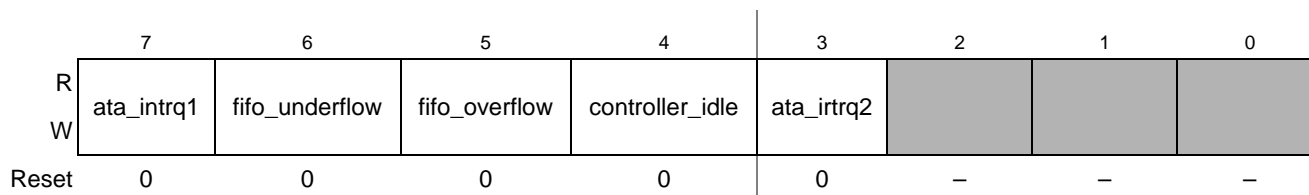
Figure 23-41. Interrupt_Enable Register
