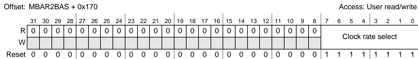
Figure 4-3. ClockRate Register
