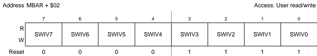
Figure 9-12. Software Watchdog Interrupt Vector Register (SWIVR)
