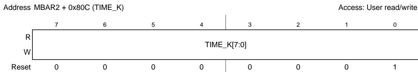
Figure 23-24. TIME_K Register
