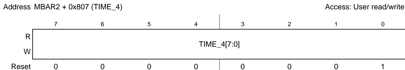
Figure 23-19. TIME_4 Register
