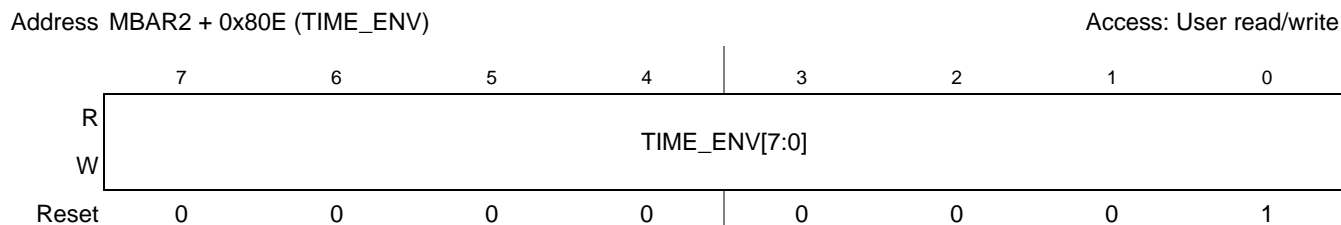
Figure 23-26. TIME_ENV Register
