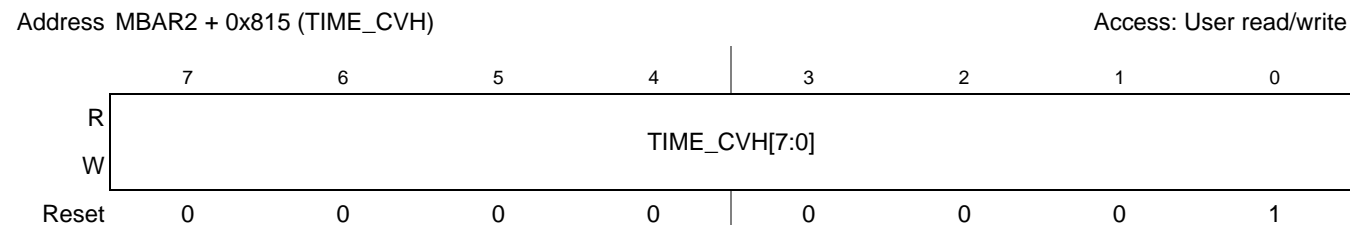
Figure 23-33. TIME_CVH Register
