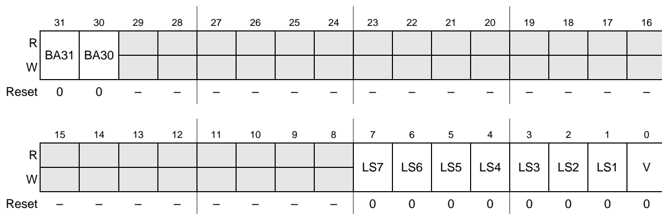
Figure 9-2. Second Module Base Address Register (MBAR2)
