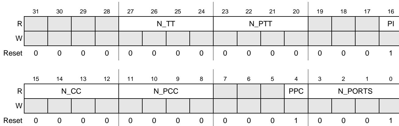
Figure 24-10. Host Controller Structural Parameters (HCSPARAMS) Register
