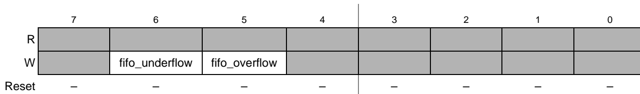
Figure 23-42. Interrupt_Clear Register
