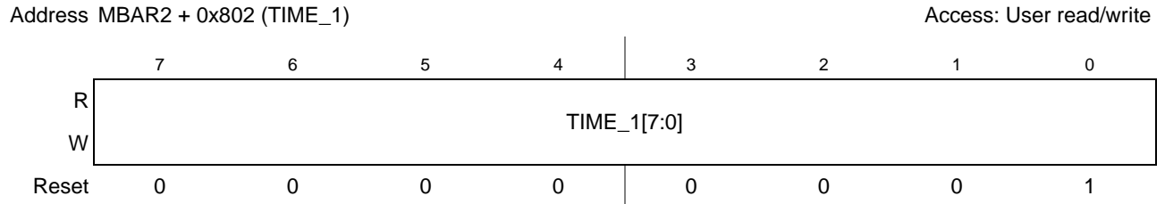
Figure 23-14. TIME_1 Register
