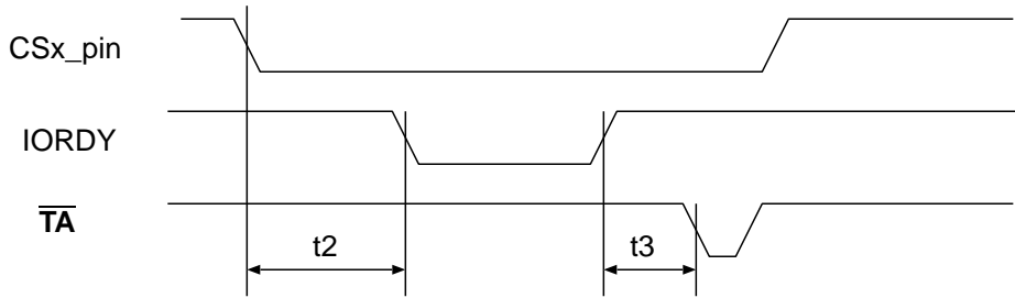
Figure 13-5. CS2 ( \overline{\text{IDE\_DIOR}} , \overline{\text{IDE\_DIO\overline{W}}} )
