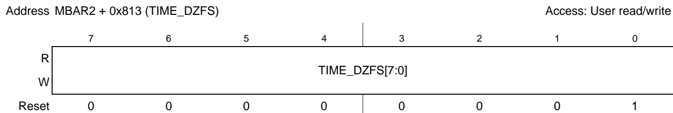
Figure 23-31. TIME_DZFS Register
