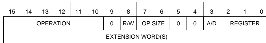
Figure 20-6. BDM Command Register
