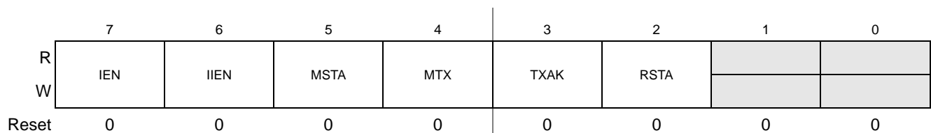
Figure 18-6. MBCR Register
