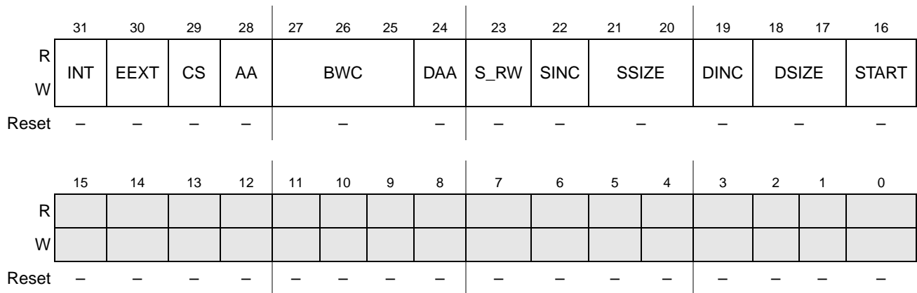
Figure 14-8. DMA Control Register (DCR)—BCR24BIT = 0
