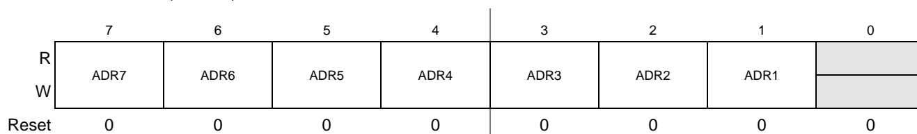
Figure 18-4. MADR Register
