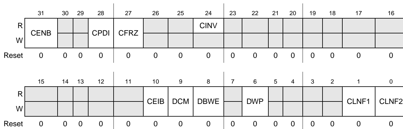
Figure 5-2. Cache Control Register (CACR)
