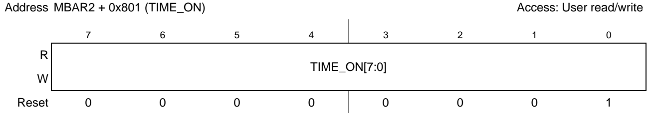
Figure 23-13. TIME_ON Register
