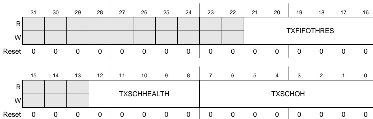
Figure 24-23. Transmit FIFO Tuning Controls (TXFILLTUNING) Register
