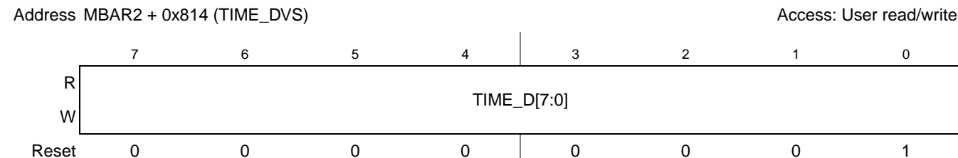
Figure 23-32. TIME_DVS Register
