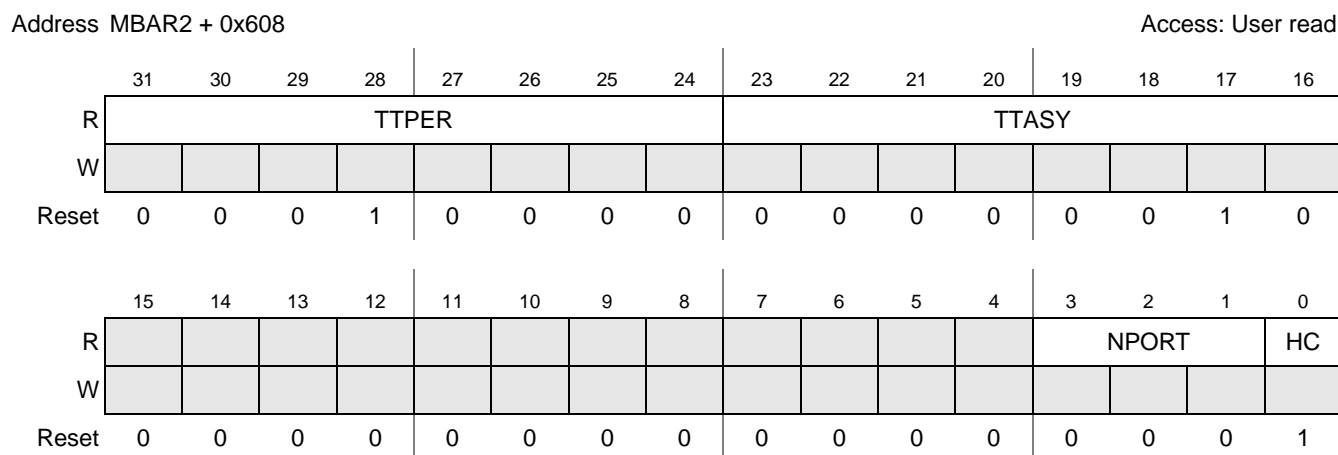
Figure 24-4. HWHOST Register
