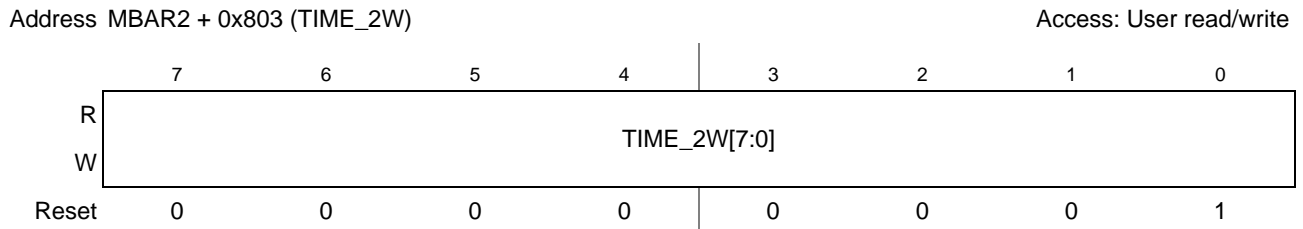
Figure 23-15. TIME_2W Register
