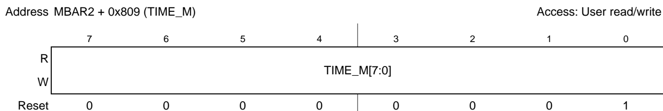
Figure 23-21. TIME_M Register
