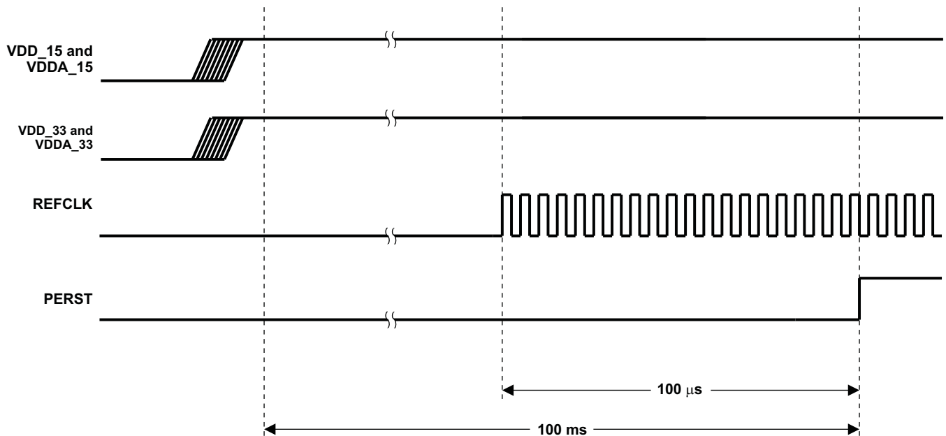
Figure 3-2. Power-Up Sequence
