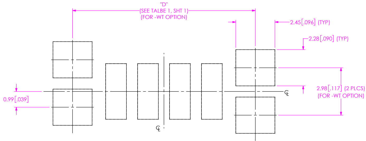
FIG 2 UMPS-04-XX.X-X-VT-SM-WT SHOWN (DIFFERENT AS SHOWN, OTHERWISE SAME AS FIG 1)
