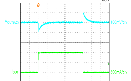
MAX17644C, 3.3V OUTPUT LOAD TRANSIENT BETWEEN 0 AND 1A, FIGURE 5 CIRCUIT
