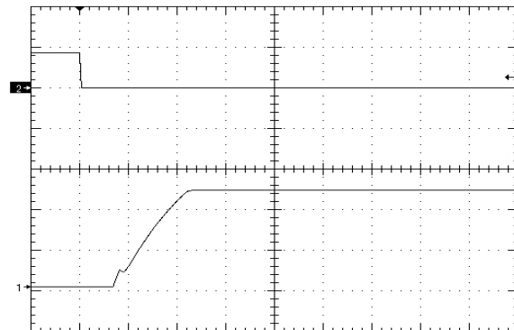
Figure 10. Startup Waveform via Enable Pin, time scale 10mS/div. Vin=Vin_nom, full resistive load + 1000µF (neg en) Ch1=10V/div, Ch2=5V/div
