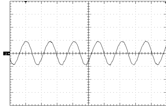
Figure 8. Input Reflected Ripple Current (20mA/div) time scale - 2µS/div. Vin=Vin_nom, full resistive.
