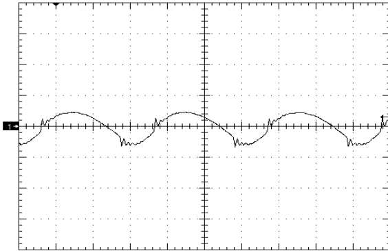
Figure 7. Output Voltage Ripple (50mV/div), time scale – 1µS/div. Vin=Vin_nom, full resistive.
