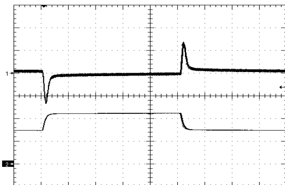
Figure 11. Load Transient Response (100mV/div), di/dt=0.1A/µS, 50% - 75% - 50% of full load, time scale: 200µS/div. Vin – 24V
