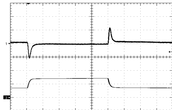
Figure 12. Load Transient Response (100mV/div), di/dt=0.1A/µS, 25% - 50% - 25% of full load, time scale: 200µS/div. Vin = 12V
