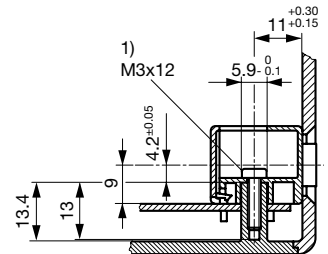
1) self tapping screw
