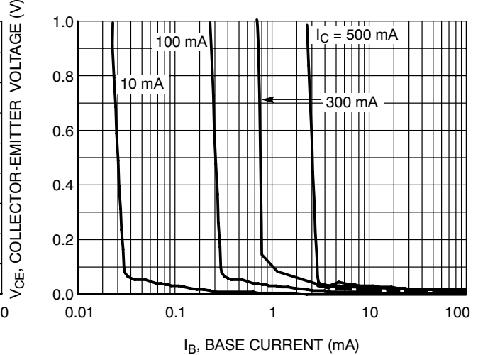
Figure 6. Saturation Region
