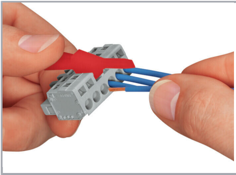
Conductor termination perpendicular to CAGE CLAMP® actuation
