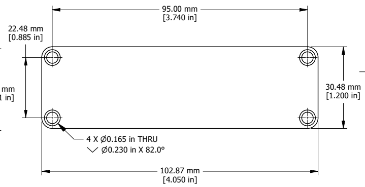
END PLATE
