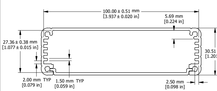
EXTRUSION
