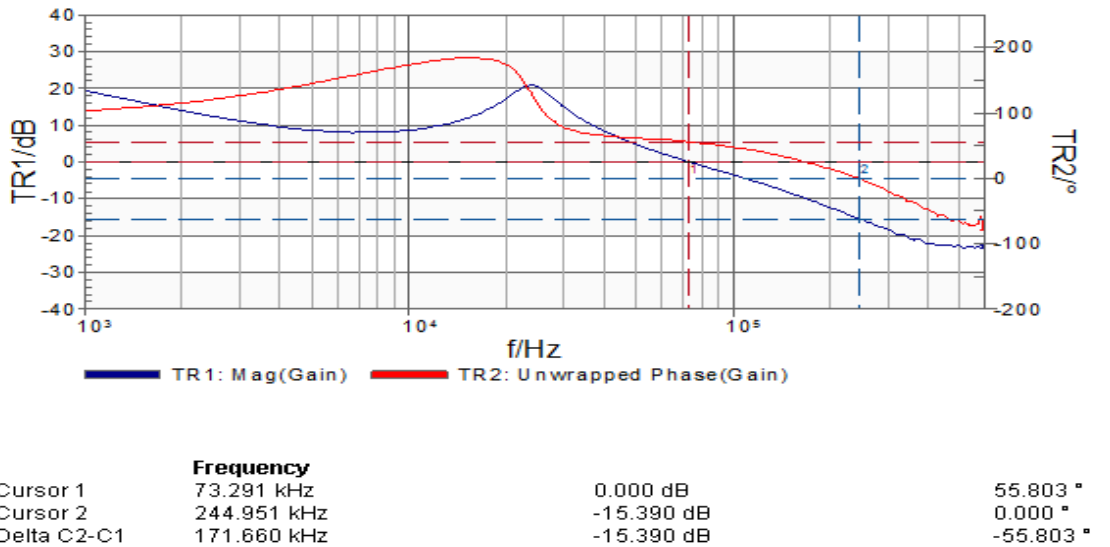
Fig. 13: Bode Plot at 35A load
