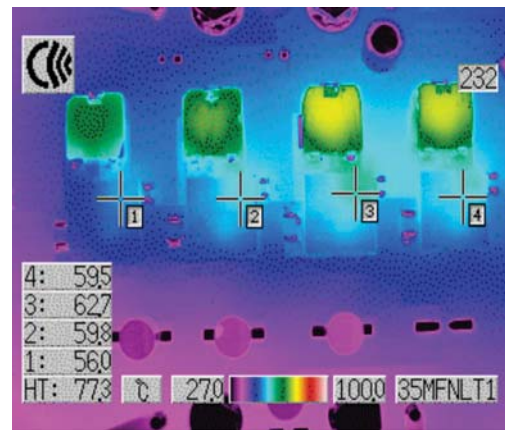
Figure 3c. Thermal Capture at 32V IN , 12V OUT , 20A, 300kHz (DC1601B-C) No Forced Airflow (Convection)
