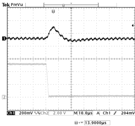
Figure 13: Typical transient response to step load change at 2.5 A/\mu s from 100% to 50% of I_o , max at 12Vin, 5.0V out ( C_{out} = 1 \mu F ceramic, 10 \mu F tantalum)
