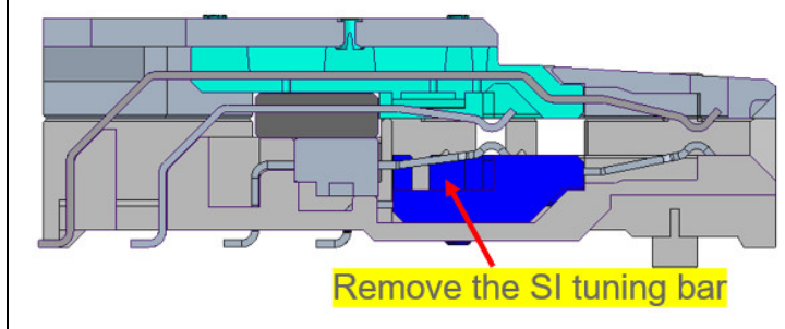
After EC, remove the SI tuning bar
