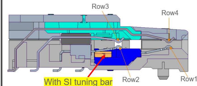
Before EC, there is a SI tuning bar between Row1 and row2 wafer
