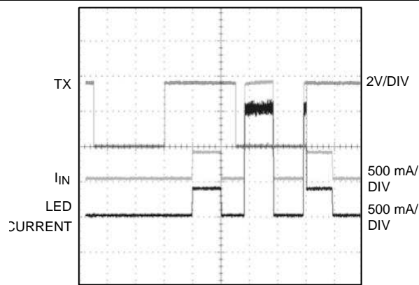
100 ms/DIV Figure 26. TX Transition Plot Behavior of LED Current Shown on Enabling the Part in a TX Event and Upon TX Interrupting During a Flash
